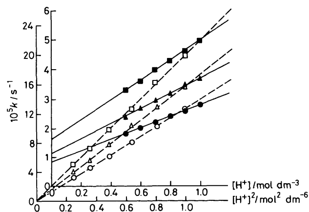
Figure 2. Acid dependence plot: k vs. [\text{H}^+] (full lines, for pbg) at 60 (●), 65 (▲), and 70 °C (■); k vs. [\text{H}^+]^2 (broken lines, for mpbg) at 60 (○), 65 (△), and 70 °C (□). [pbg] = 0.05, [mpbg] = 0.01, [Cr VI ] = 0.1, and I = 2 \text{ mol dm}^{-3} .
